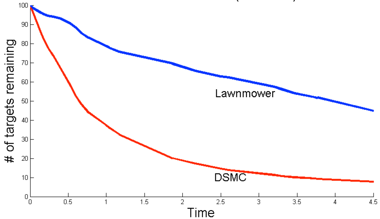
DSMC vs Lawnmower (Gaussian)
